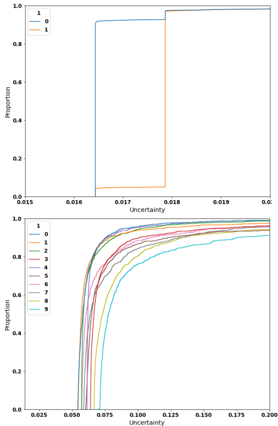
Figure 2: Cumulative evidential signal of samples split by the ground-truth label for IMDB (top) and MNIST (bottom).
