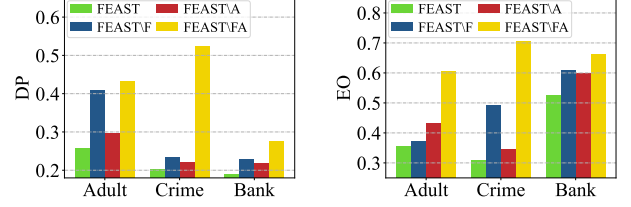
Figure 2: Ablation study on our framework FEAST on three datasets under the 5-shot setting.
