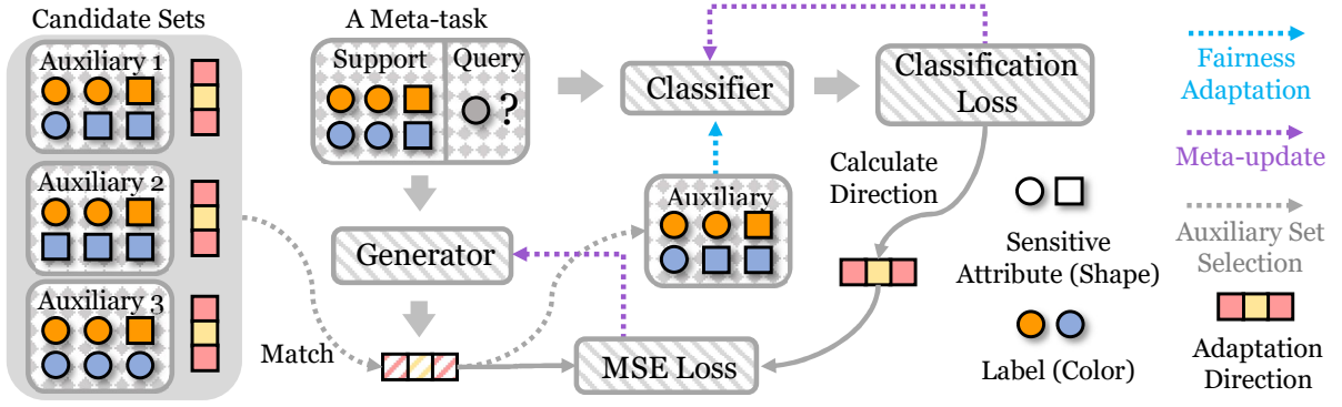
Figure 1: The overall process of our proposed framework FEAST. Here different shapes denote different sensitive attributes, and colors represent sample classes. Given a meta-task, the generator will output the estimated fairness adaptation direction, which is used to select an auxiliary set with the most similar direction from the candidate set. Then we conduct fairness adaptation with the auxiliary set on the current meta-task and perform predictions. The resulting fairness adaptation will be used to update the generator. Note that during training, the meta-task will be incorporated into the candidate auxiliary sets after the optimization of one episode.
