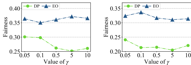
Figure 3: Results of FEAST on Adult (left) and Crime (right) with different values of \gamma .
